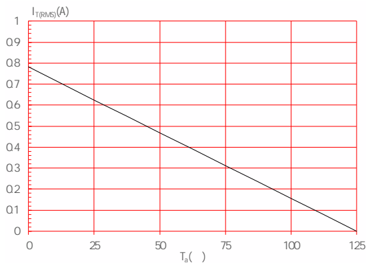
On-state characteristics
